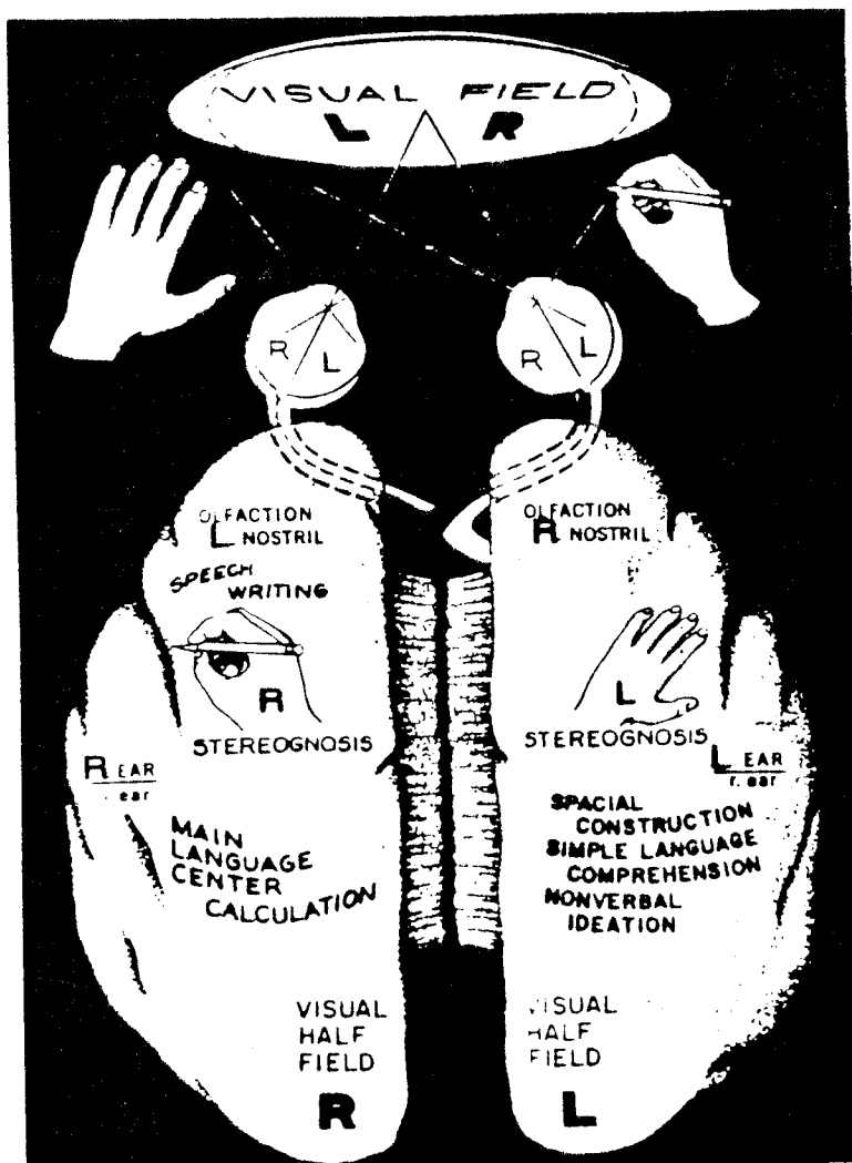
FIG. 2. Schematic representation of some of the main cerebral functions found to be lateralized following hemisphere disconnection.
