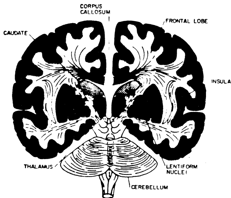
FIG. 1 Nature of hemispheric separation effected by surgical section of forebrain commissures. Some indirect cross communication remains possible through intact midbrain and associated brainstem structures.
