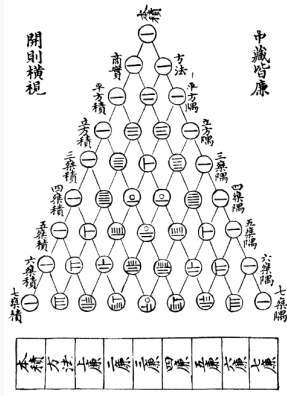
Figure 5: Jia Xian triangle published in 1303 by Zhu Shijie
