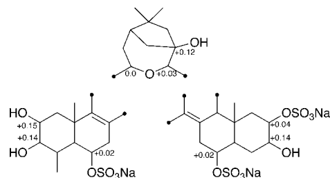
Figure 2. Selected deuterium-induced isotope shifts in the 13 C NMR spectrum of amaroxocane A (1). \delta\delta = [\delta_C(\text{CD}_3\text{OD}) - \delta_C(\text{CD}_3\text{OH})] .
