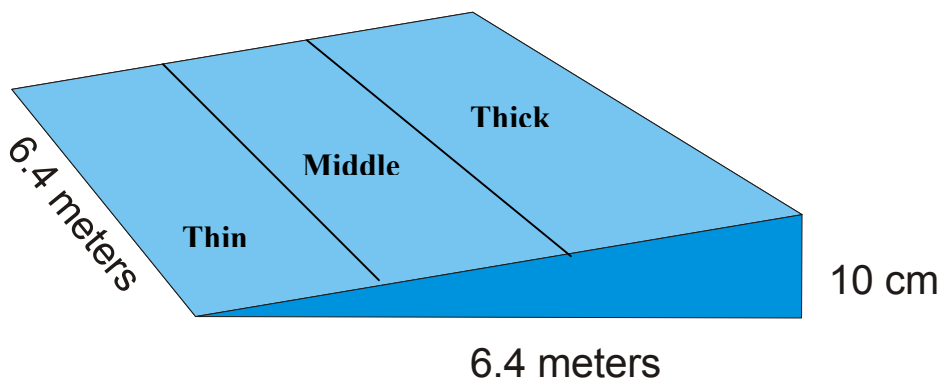
Figure 3. Diagram showing geometry of sediment fill.
