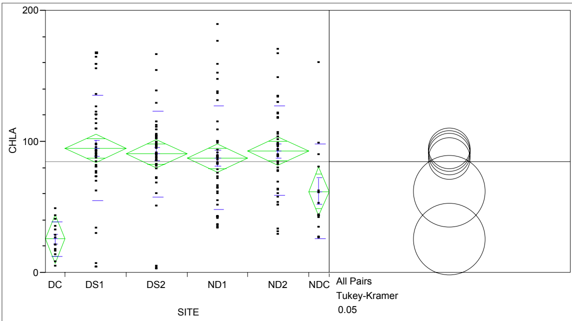
Figure 17. Comparison of Chl a mean and variability in amended and control sites.
