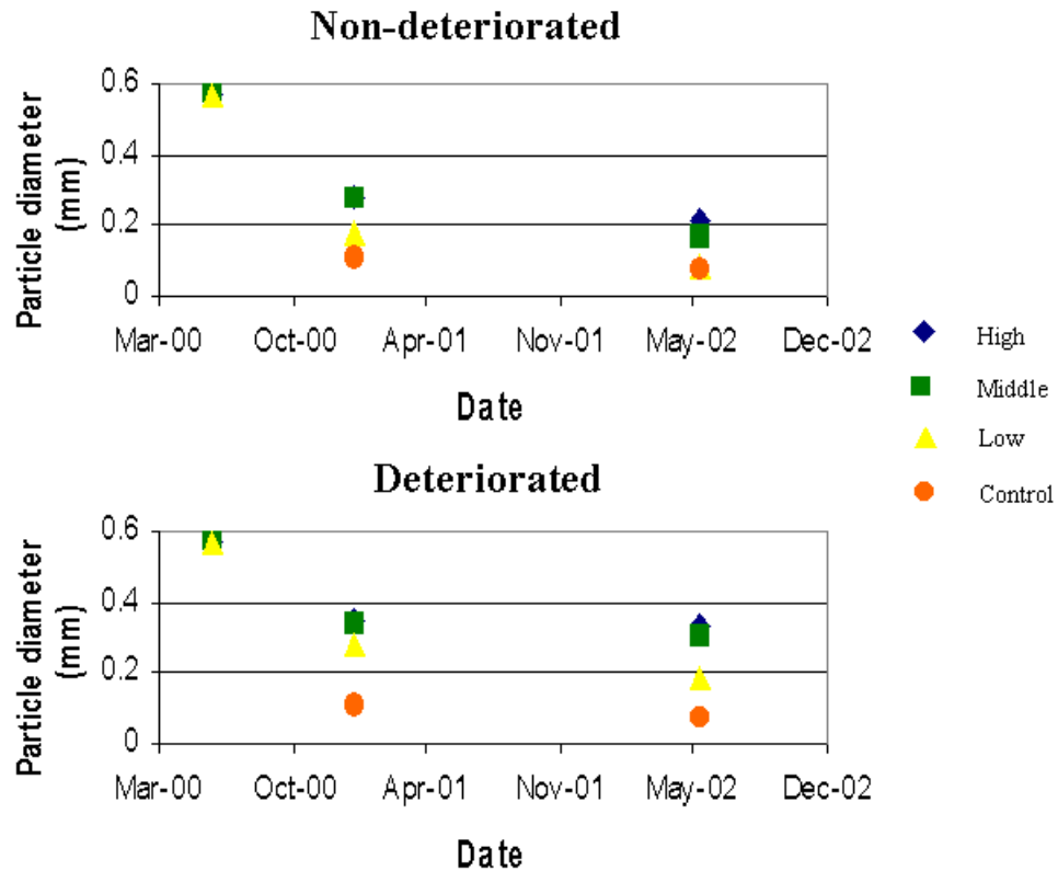
Figure 13. Surficial mean grain size for the deteriorated and non-deteriorated sties.
