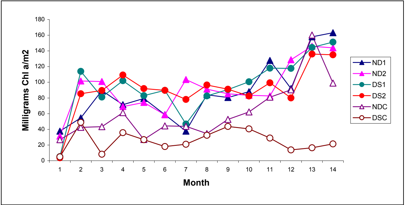
Figure 16. Comparison of mean monthly Chl a of amended sites versus control sites. ND indicates amended non-deteriorated sites, DS indicates amended deteriorated sites, and NDC and DSC indicate non-deteriorated and deteriorated control sites, respectively.
