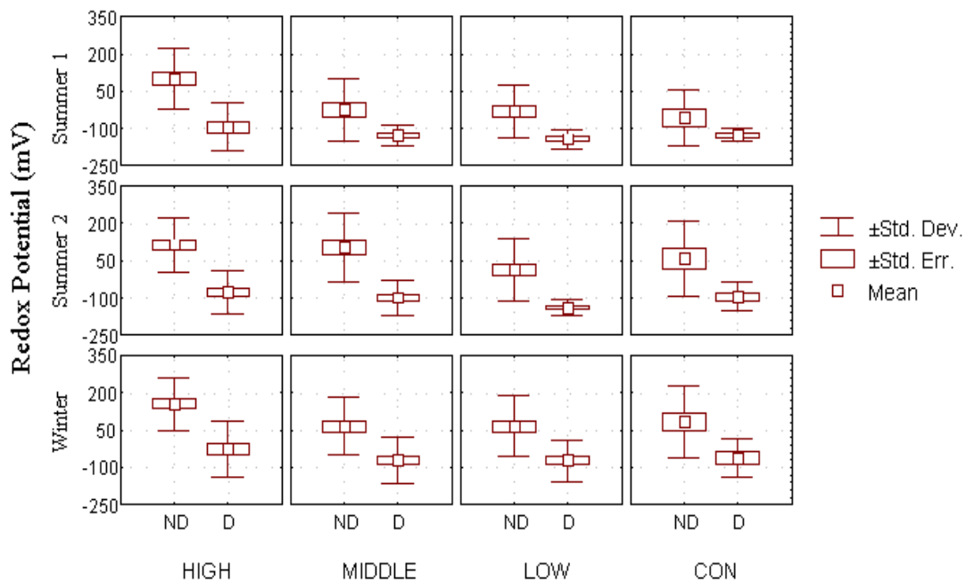
Figure 10. Box plots – Treatment versus seasonality versus marsh type.
