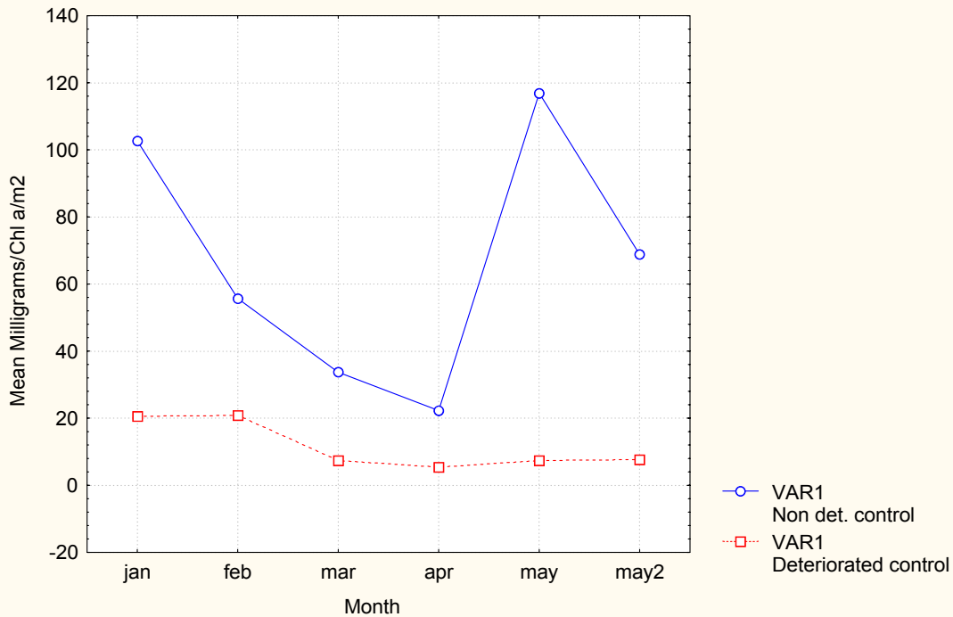
Figure 15. Mean Chl a of pre-sedimented sites/month.
