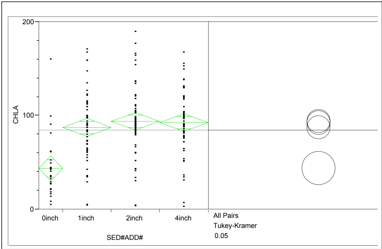
Figure 19. Comparison of Chl a means and variability among amended sites resulting from incremental sediment additions.
