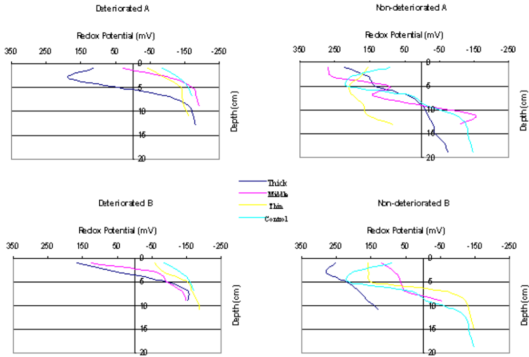
Figure 8. Averaged eH profiles for each study site (Aug 2000 – Nov 2001).
