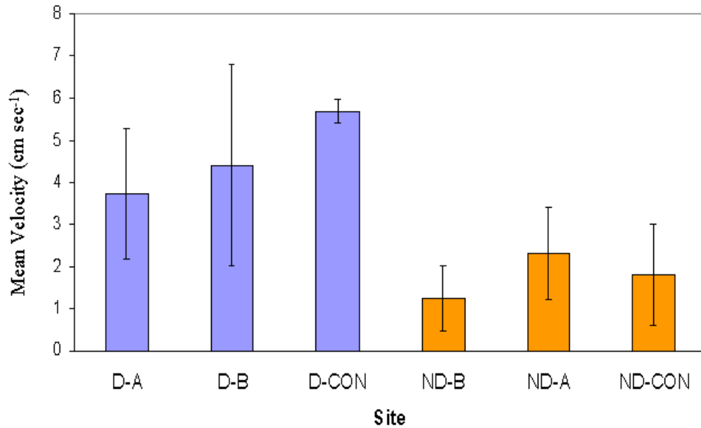
Figure 14. Mean flow velocities for the deteriorated and non-deteriorated sites. Each mean is calculated from three sampling bursts. Error bars indicate \pm one standard deviation for the three sampling bursts.
