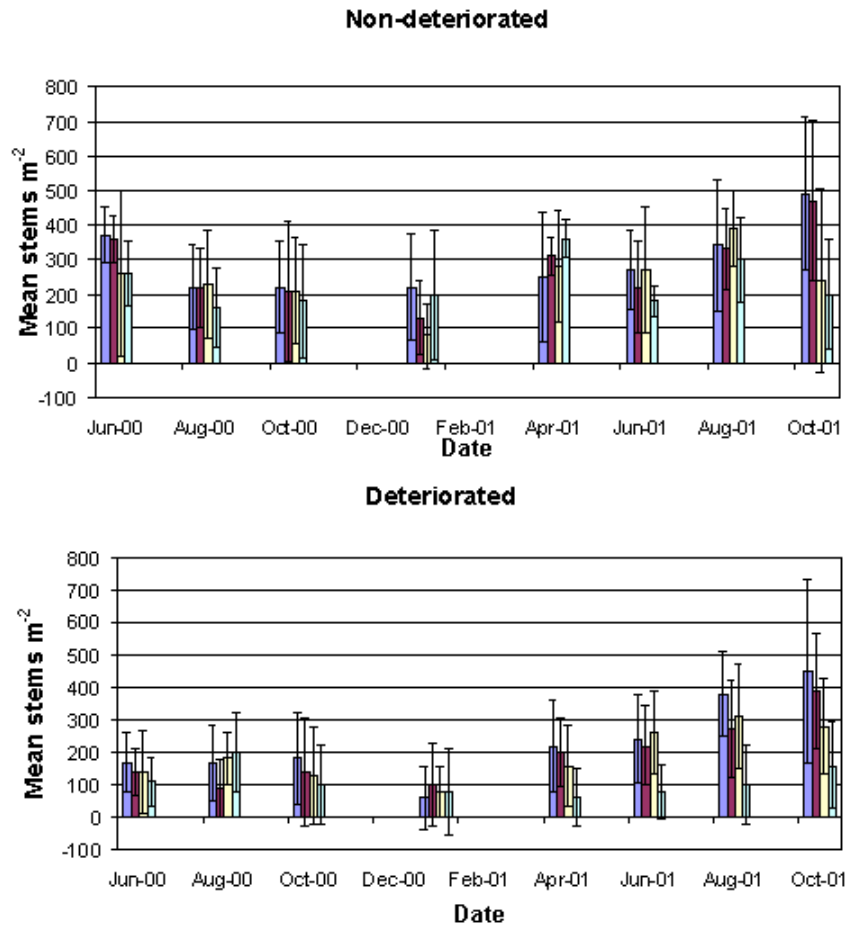
Figure 4. Mean stem densities of Non-deteriorated and Deteriorated sites. Thick treatments are shown in blue, medium treatments in red, thin treatments in yellow, and controls in aqua. Error bars indicate \pm one standard deviation.
