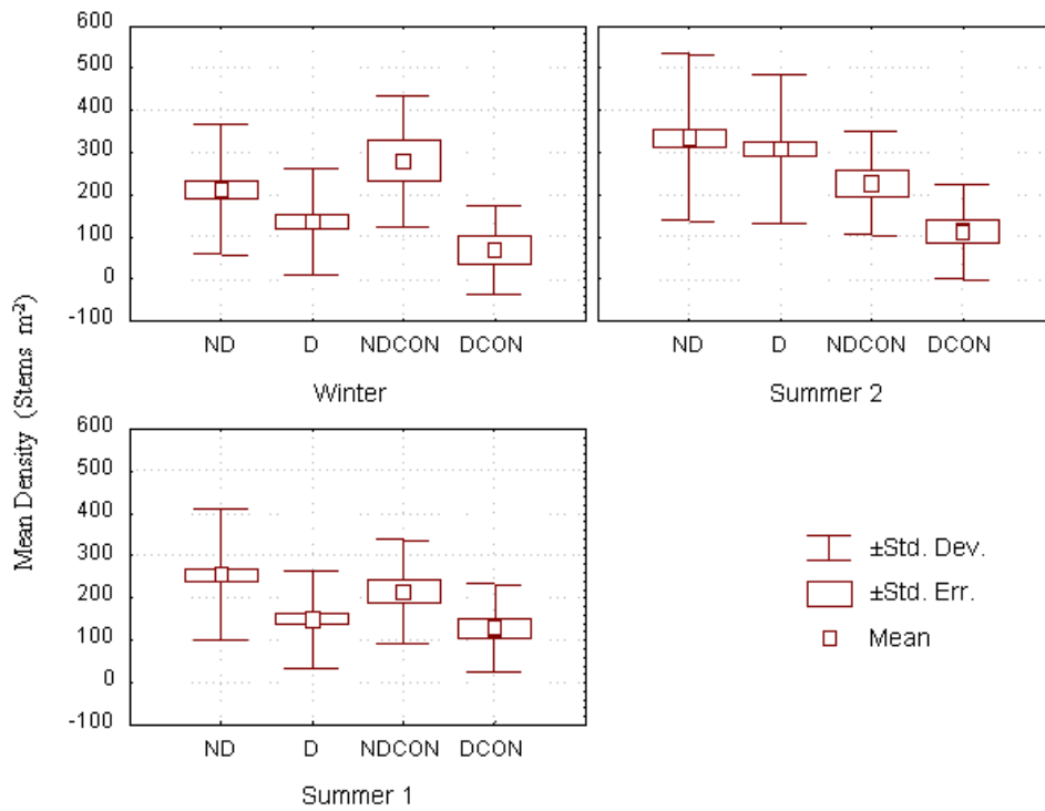
Figure 5. Box plots showing mean seasonal stem densities for non-deteriorated, deteriorated, and control sites.
