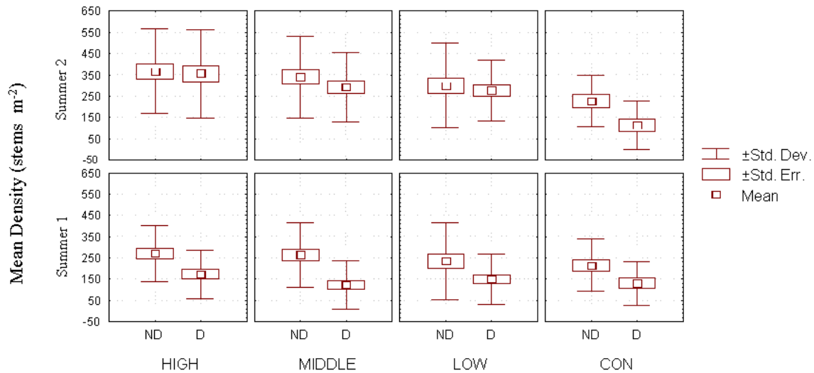
Figure 6. Whisker box plots of mean stem densities by treatment level in Summer 1 and Summer 2.
