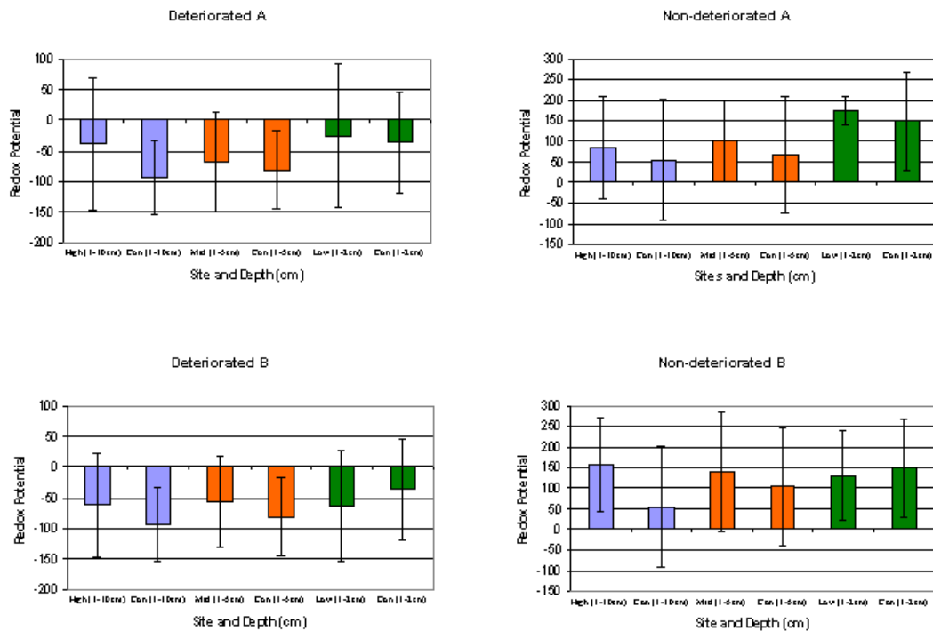
Figure 11. Mean depth-integrated Redox potentials measured within the sediment addition layer and an equivalent depth in the associated control. Error bars indicate \pm one standard deviation of the mean. A high degree of seasonal variation and the decreasing exponentially shape of the profiles account for the large standard deviations shown.
