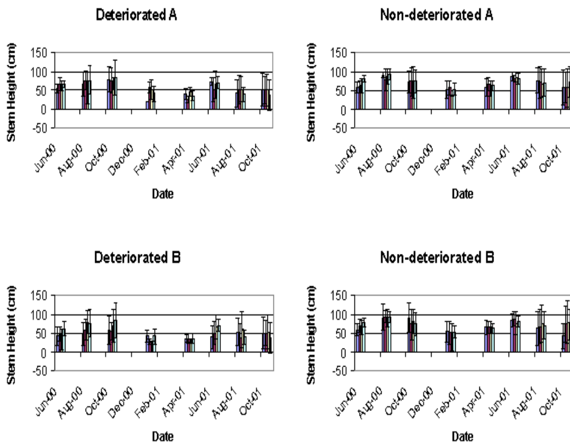
Figure 7. Monthly mean plant heights for various treatments in deteriorated and non-deteriorated marsh types. Thick treatments are shown in blue, medium treatments in red, thin treatments in yellow, and controls in aqua. Error bars indicate \pm one standard deviation.
