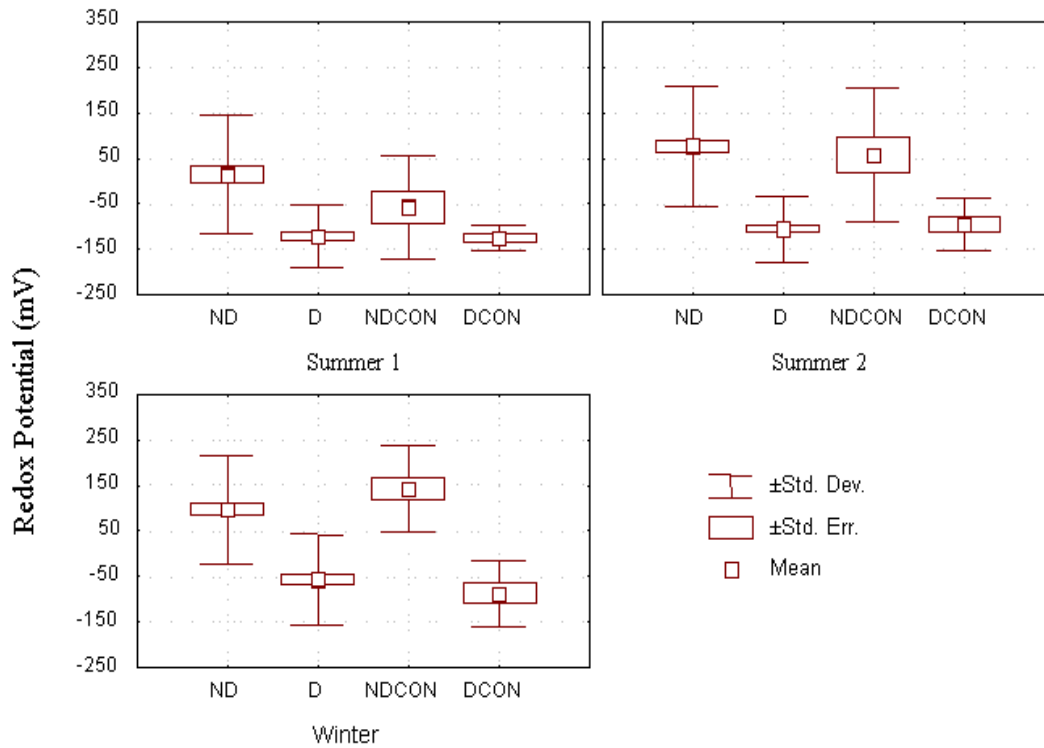
Figure 9. Seasonal box plots for treated (averaged) and control non-deteriorated and deteriorated sites.
