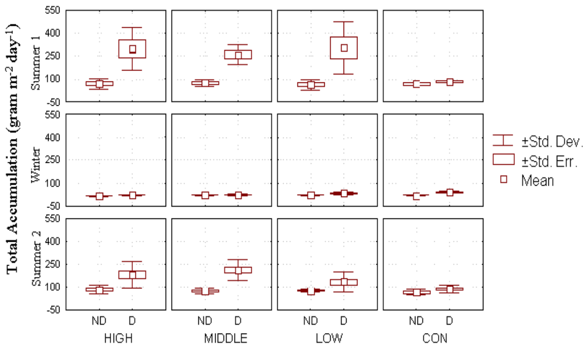
Figure 12. Surficial sediment deposition measured in deteriorated (D) and non-deteriorated (ND) experimental marsh sites.
