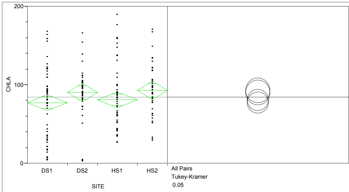
Figure 18. Comparison Chl a means and variability between deteriorated and non-deteriorated sites post sediment addition.
