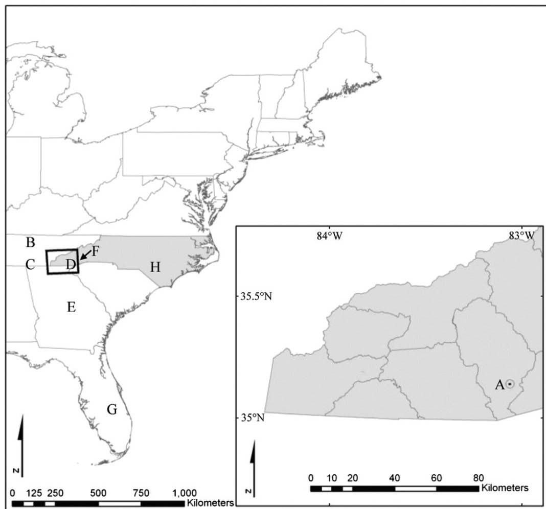
Figure 1. Map of the eastern United States showing the location of the Panthertown Valley site (Site A on inset, 35°09.55' N, 83°01.30' W) within Jackson County, NC. Other sites discussed in the text are also represented including Anderson Pond (B), Raccoon Mountain Cave (C), Horse Cove Bog (D), Sandy Run Creek (E), Flat Laurel Gap (F), Lake Tulane (G) and the Little River Site (H).
