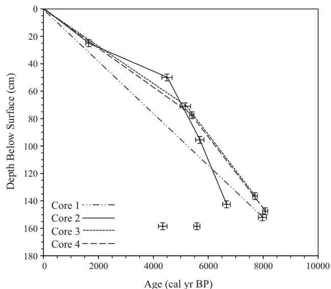
Figure 2. Age–depth model for the Panthertown site. All radiocarbon dates from cores 1–4 are plotted vs. depth. X-axis error bars ( 2\sigma ) and y-axis error bars (5 cm sample thickness) are shown. Specific age/depth information with respect to individual cores is presented in Table 1. The lines on the graph show changes in the sedimentation rate and connect the data points for each core separately. These lines are forced through zero. The two radiocarbon dates that are out of stratigraphic order are shown on the graph but are not connected by a line.
