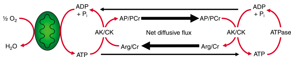
Fig. 2. Phosphagen kinases (AK or CK) mediate most diffusive flux of ATP in muscle. The red arrows indicate enzymatic catalysis and the black arrows net diffusive flux. The relatively thick black arrows for phosphagen kinase mediated diffusion indicates that the vast majority of net high-energy phosphate diffusion occurs in the form of phosphagen (AP or PCr), rather than directly as ATP (thin black arrows).
