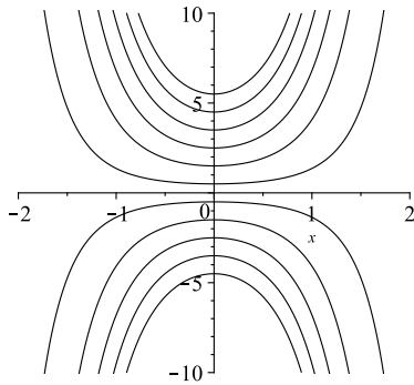
Figure B.1: Plots of solutions from the 1-parameter family of solutions of Example B.1 for several initial conditions.
