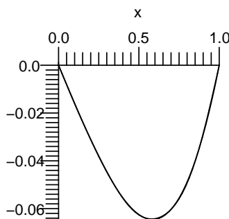
Fig. 8.4. Plots of the exact solution to Example 8.5 with the first five terms of the series solution.
