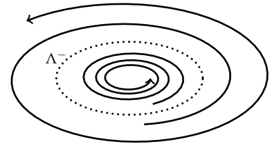
Figure 7.34: A sketch depicting an \alpha -limit set. Note that the orbits tend away from the set as t increases.
