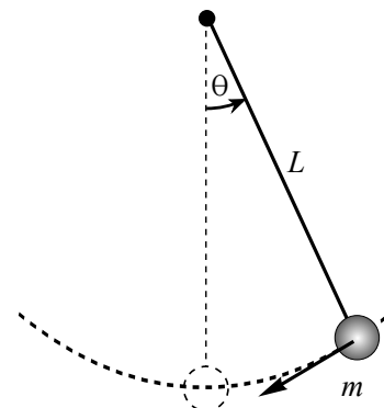
Figure 7.10: A simple pendulum consists of a point mass m attached to a string of length L . It is released from an angle \theta_0 .
