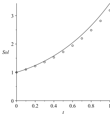
Figure 3.2: A comparison of the results Euler's Method to the exact solution for y' = x + y , y(0) = 1 and N = 10 .
