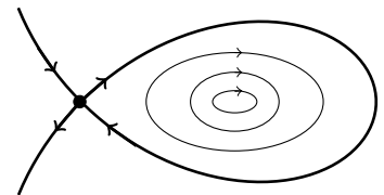
Figure 7.36: A homoclinic orbit returning to the point it left.
