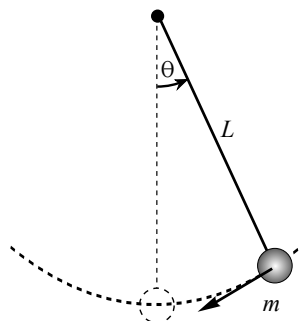
Figure 2.2: A simple pendulum consists of a point mass m attached to a string of length L . It is released from an angle \theta_0 .
