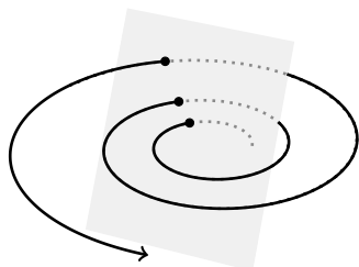
Figure 7.43: As an orbit pierces the surface of section, one plots the point of intersection in that plane to produce the surface of section plot.
