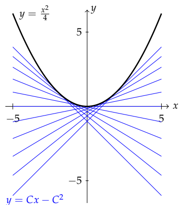
Figure 1.5: Plot of solutions to the Clairaut equation y = xy' - y'^2 . The straight line solutions are a family of curves whose limit is the parametric solution.
