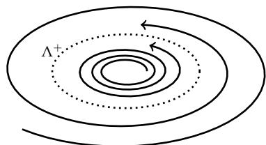
Figure 7.33: A sketch depicting an \omega -limit set. Note that the orbits tend towards the set as t increases.
