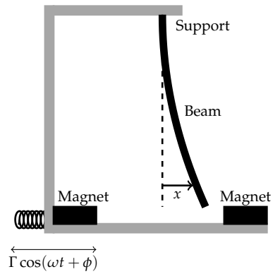
Figure 7.37: One model of the Duffing equation describes a periodically forced beam which interacts with two magnets.
