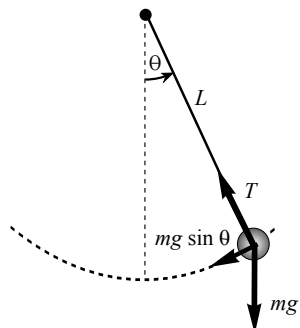
Figure 2.3: There are two forces acting on the mass, the weight mg and the tension T . The net force is found to be F = mg \sin \theta .
