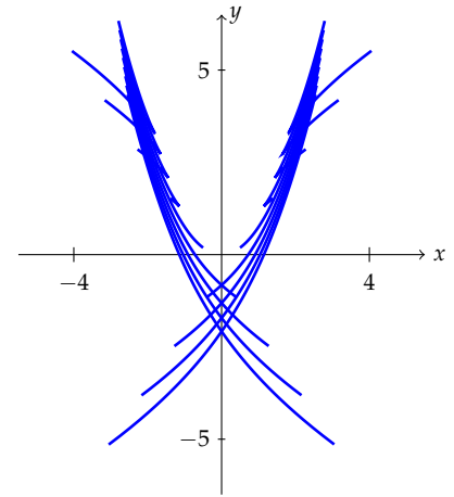
Figure 1.4: Family of solutions of the Lagrange equation y = 2xy' - y'^2 .
