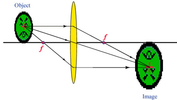
Fig. 1: Ray trajectories for a convex lens
