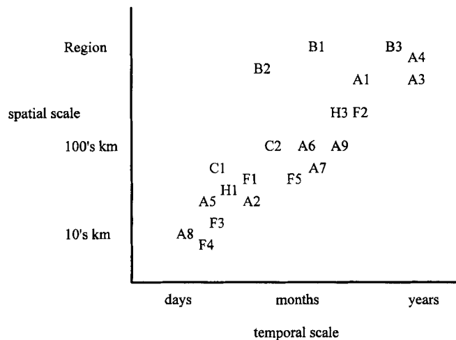
Fig. 3. Temporal and spatial scales for CEMP parameters. Refer to Table I for an explanation of the parameter labels. For example, penguin chick diet (A8) would be expected to reflect local krill availability over the days that an adult penguin is away on a foraging trip; whereas penguin adult weight on arrival at a breeding colony (A1) would be expected to reflect krill abundance and availability in the ISR for several months prior to breeding. H2 has identical characteristics to H1.
