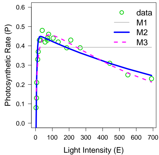
Figure 1: Example of fitting alternative process models to laboratory data for the relationship between photosynthesis ( P ) and light irradiance ( E ).
