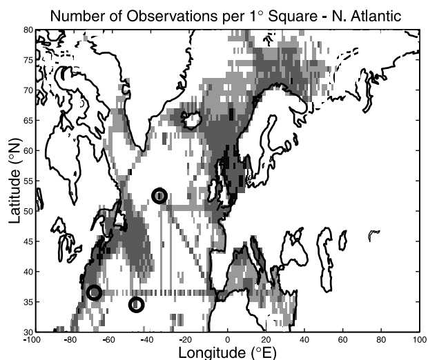
Figure 3. Number of historical SSS observations per 1° square in the North Atlantic. Note slightly different scale from Figure 2. Light gray, ≥30 observations; dark gray, ≥100 observations; and black, ≥1000 observations. No fill means less than 30 observations. Dark circles at (35.5°W, 52.5°N), (69.5°W, 36.5°N), and (47.5°W, 34.5°N) are squares listed in Table 2 and have details of data distribution shown in Figures 4a–4c.
